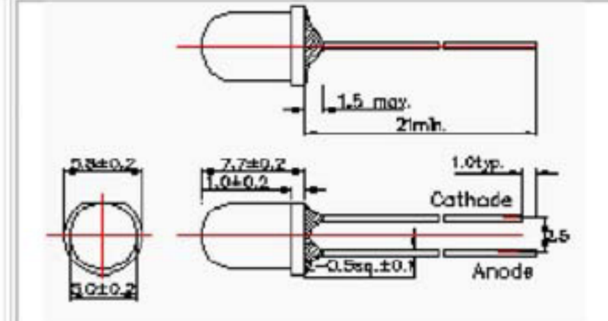
Figure 6 Ö5 Mold type 06
