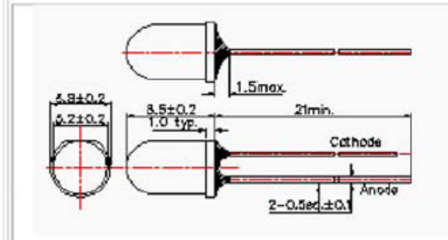
Figure 4 Ö5 Mold type 04
