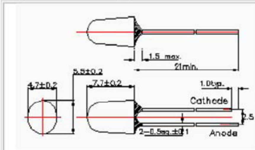
Figure 9 Ö3 Mold type 33
