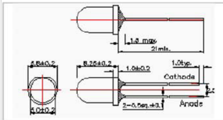
Figure 5 Ö5 Mold type 05
