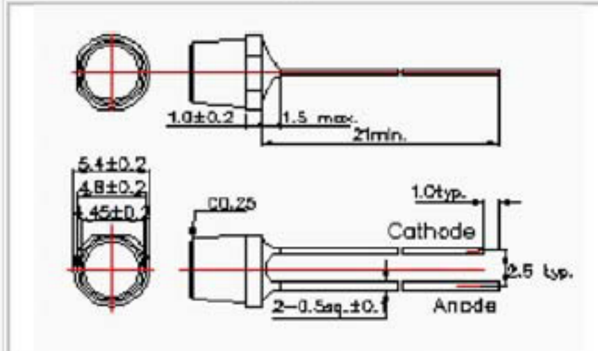
Figure 7 Ö5 Mold type 09
