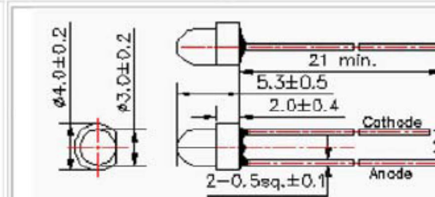
Figure 10 Ö3 Mold type 36
