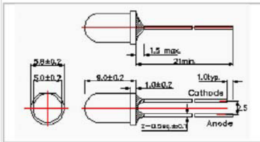
Figure 3 Ö5 Mold type 03
