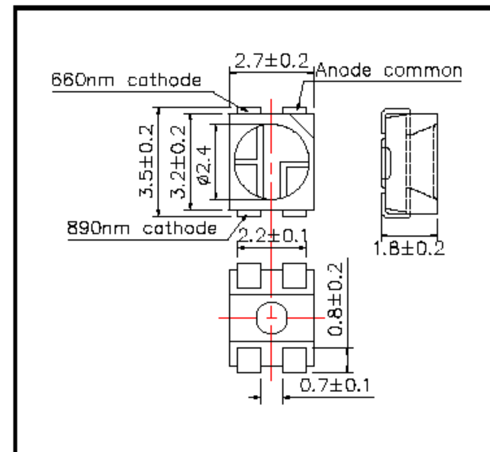
◆ Outer dimension (Unit:mm)
